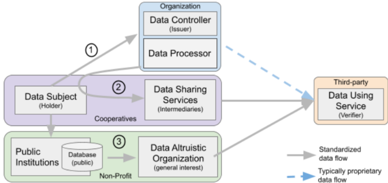
Figure 1: Data Governance Act Architecture Overview
